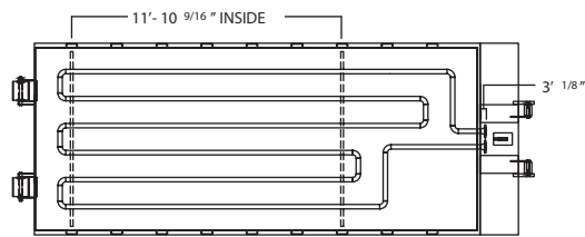
Top View (with coils)
