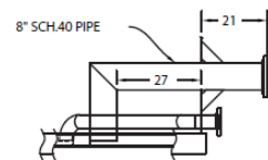
1290-0013 External Manifold Details
