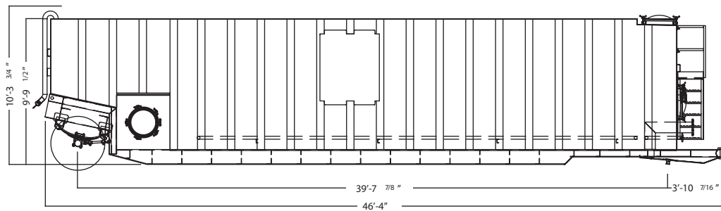
Side View
