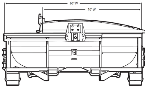
Roof shown front closed
